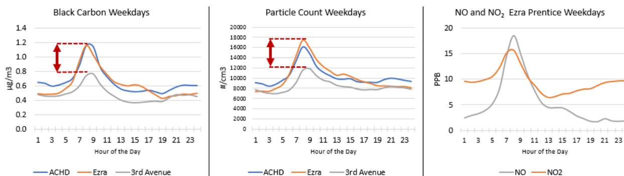
Figure 26. Weekday Diurnal Plots for Nitrogen Oxides, Black Carbon, Ultrafine Particles
