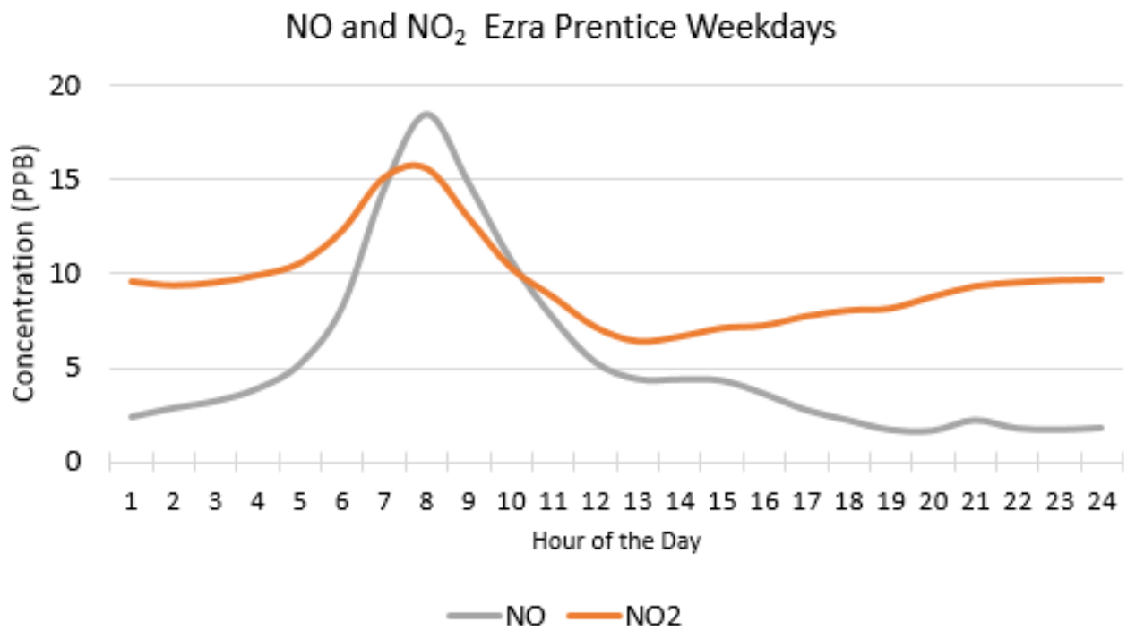
Figure 15. Nitrogen Oxides Diurnal Plots Weekdays Fixed
