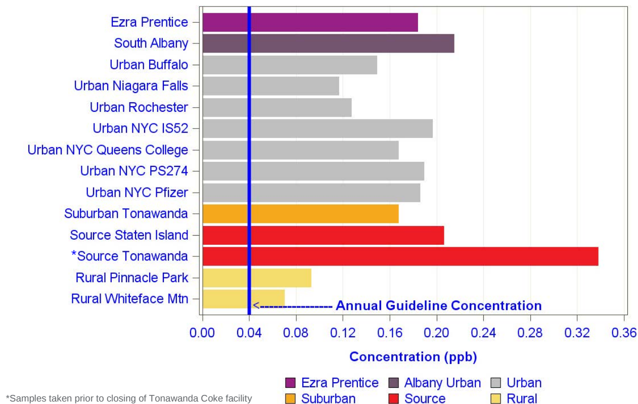
Figure 20. Benzene Annual Average Ezra Prentice and South Albany compared to NYSDEC Network Monitors
