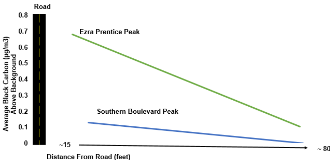
Figure 51. Average Peak Black Carbon Concentrations above Background at Ezra Prentice and Southern Boulevard
