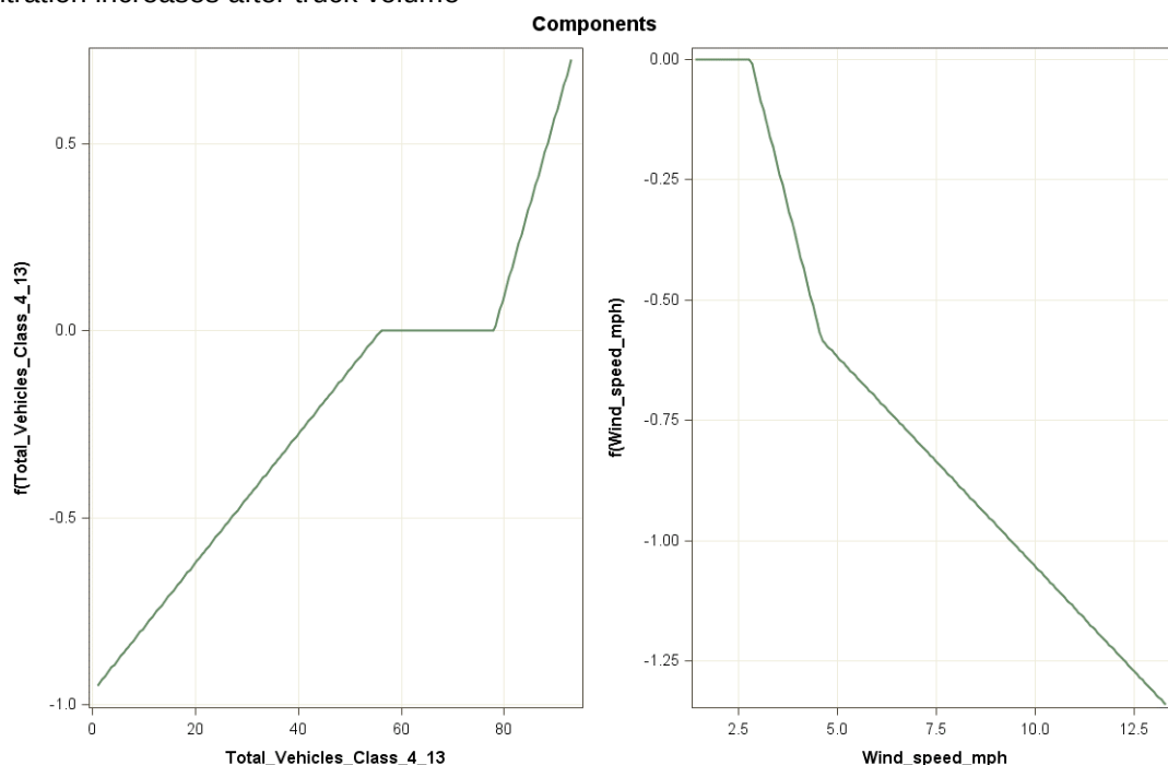
Figure 4. UFP Counts Modeled Relationship to Independent Variables
