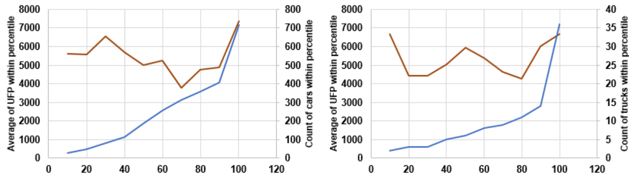
Figure 30. Sunday Percentile Comparison Total Cars (left, blue) and Trucks (right, blue) with UFP (red)
